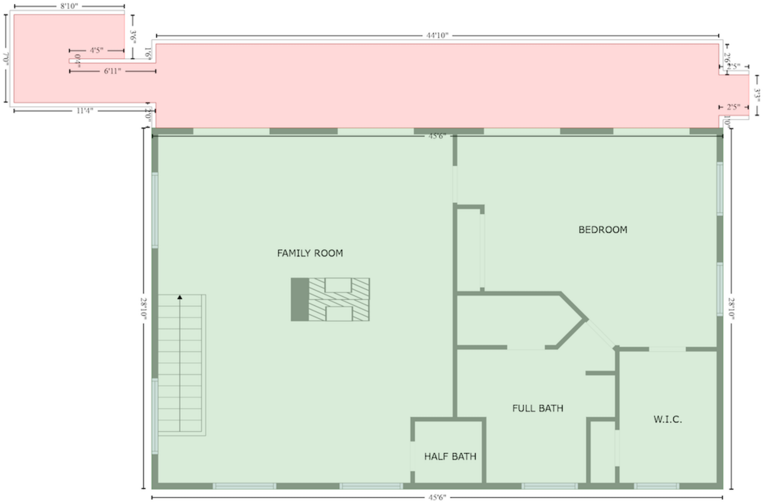
FLOOR 3 [AREA: 1310]
